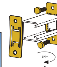
TYPE INC8
