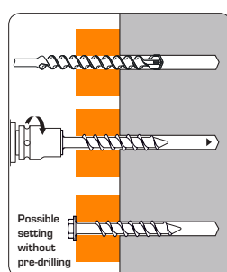
ACS HEX Installation
