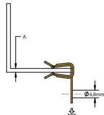
TYPE H
