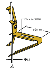
TYPE Z-CTS
